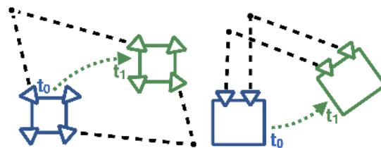
Figure 1. Illustration of moving multi-camera rigs. The black points and dashed lines indicate corresponding observations of a feature in the two capture instances. Left : A general multi-camera configuration with four cameras. Right : An axial camera configuration with two cameras (a stereo camera).
