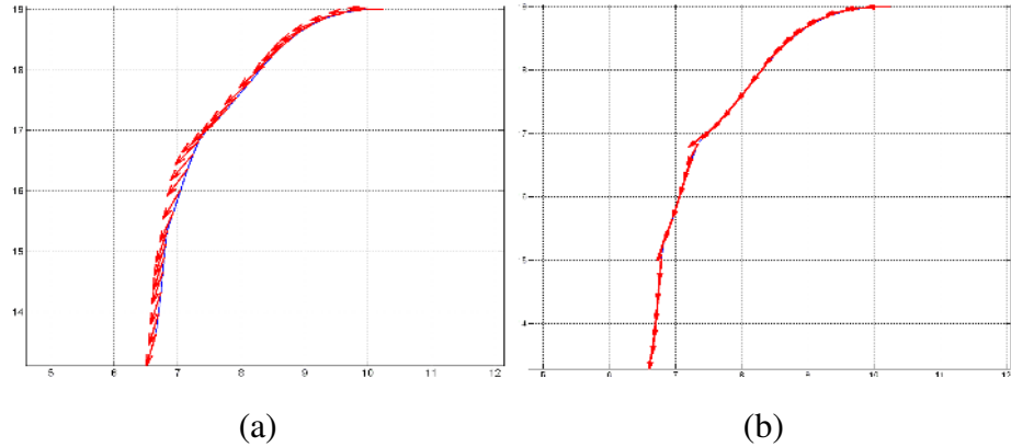
Figure 18. Recovered 2D trajectory of the subject of Fig. 17. The underlying grid is made of 1x1 meter squares and the arrows represent the direction he is facing. (a) When orientation and motion are not linked, he appears to walk sideways. (b) When they are, he walks naturally.
