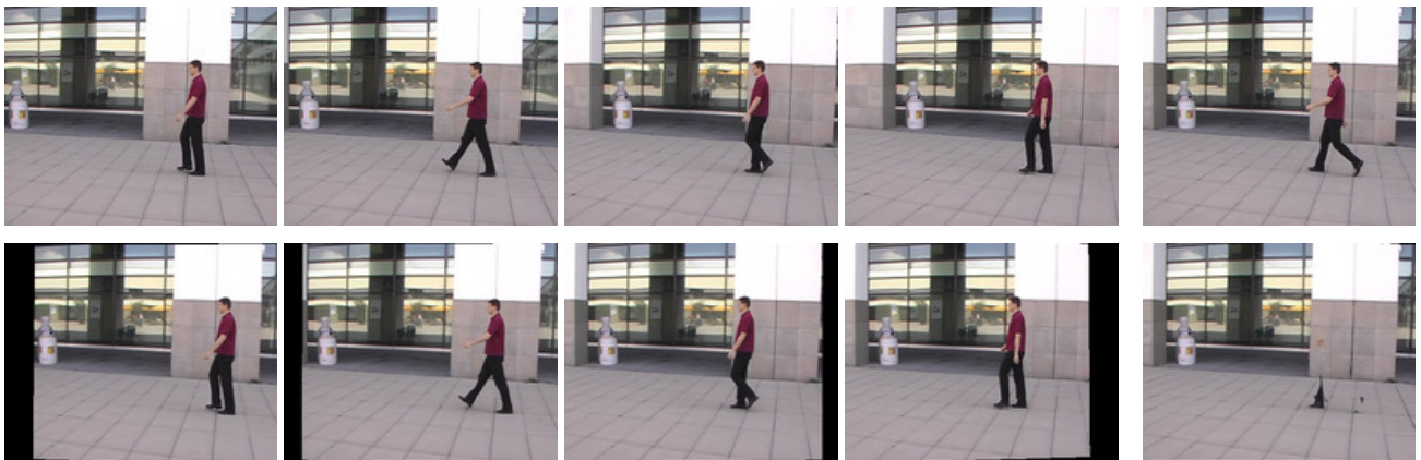
Figure 11. Synthesizing a background image. First row: The rightmost image is the reference image whose background we want to synthesize. The other 4 are those before and after it in the sequence. Second row: The same four images warped to match the reference image. Computing the median image of these and the reference image yields the rightmost image, which is the desired background image.
